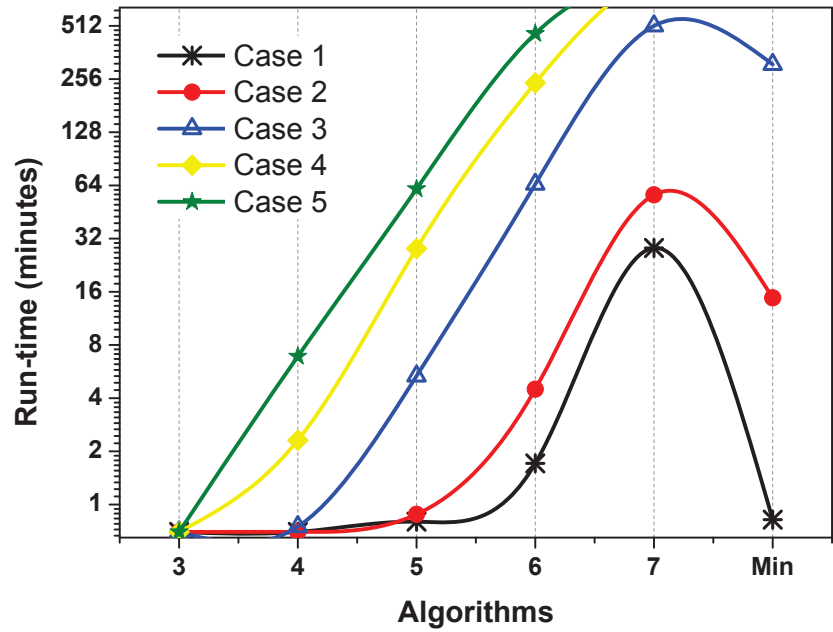
Figure 10: Running time comparing different fault tree analysis algorithms. 3 – 7 located at X-axis are used to denote failure sampling algorithm at various powers of 10. Min represents the minimal cut set algorithm.
